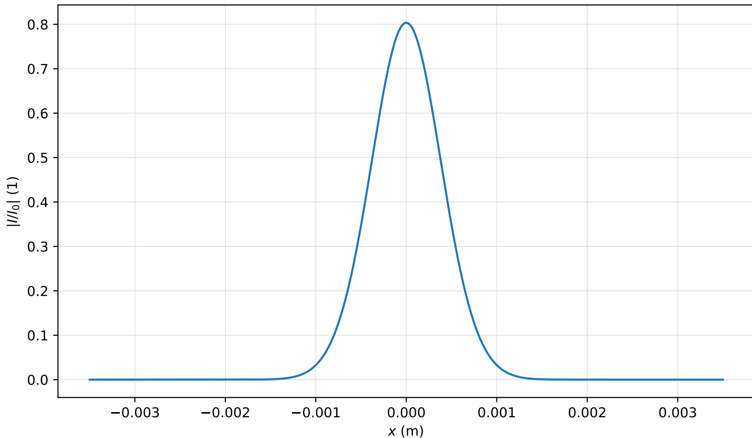
Intensity profile I(x, y = 0, z = 1.115m)/I_0 , P_{in}=0.1P_{cr} , artificial time
